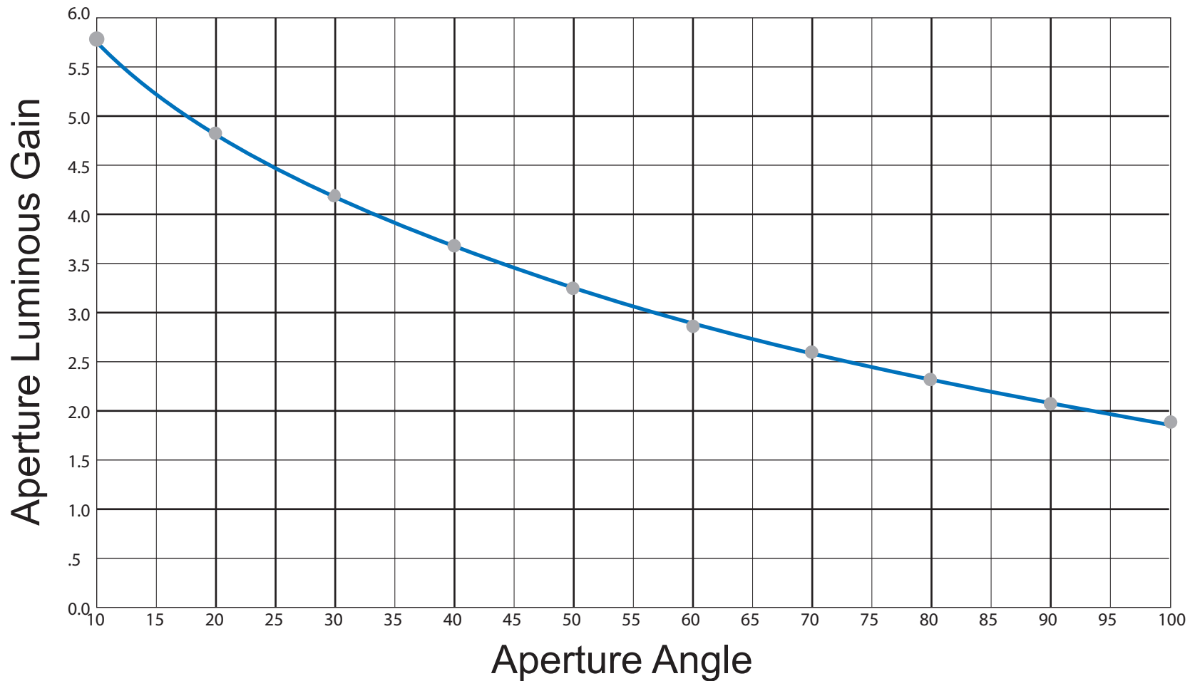
Aperture Angle vs. Aperture Luminous Gain
