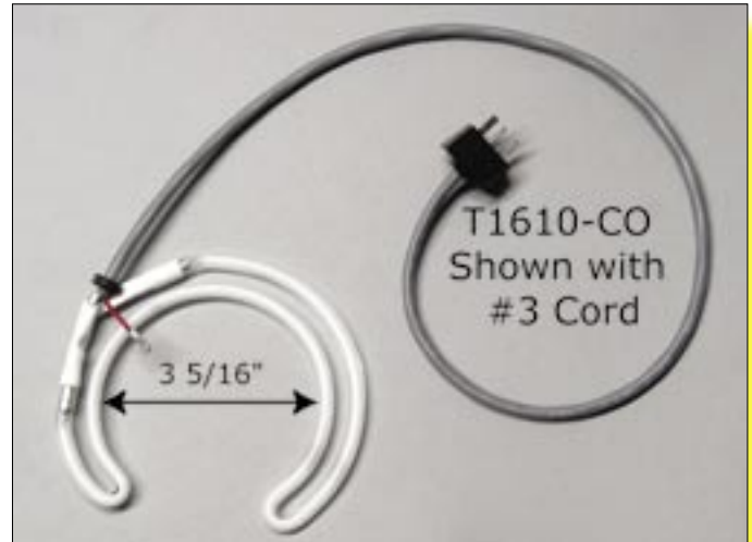
Cut Out Replacement Lamp Head Assembly: Lamp, Power Cord and 3 pin rectangular connector
